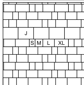
Pattern BE.31 - Small 105x140mm - 8 Medium 140x140mm - 8 Large 210x140mm - 8 XLarge 252x140mm - 8 Jumper 280x210mm - 5
