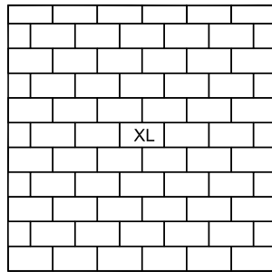
Pattern BE.6 - XLarge 252x140mm - 28
