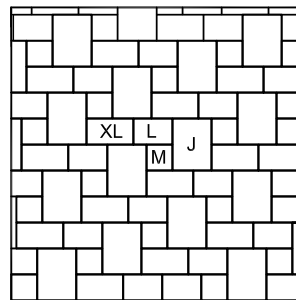
Pattern BE.15 - Medium 140x140mm - 7
