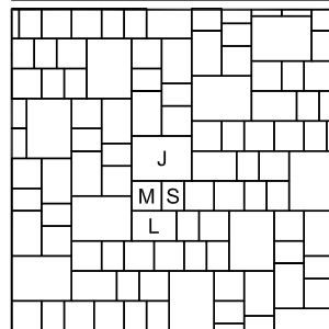
Pattern BE.30 - Small 105x140mm - 15 Medium 140x140mm - 15 Large 210x140mm - 8 Jumper 280x210mm - 5
