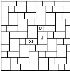
Pattern BE.21 - Medium 140x140mm - 9 XLarge 252x140mm - 9 Jumper 280x210mm - 9
