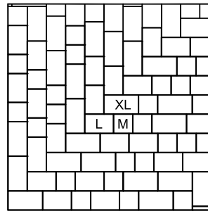
Pattern BE.11 - Medium 140x140mm - 12
