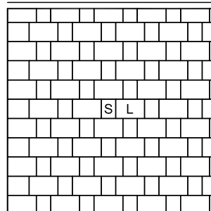
Pattern BE.34 - Small 105x140mm - 23 Large 210x140mm - 23
