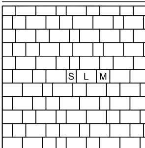
Pattern BE.33 - Small 105x140mm - 6 Medium 140x140mm - 12 Large 210x140mm - 24
