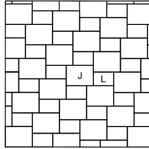
Pattern BE.18 - Large 210x140mm - 12 Jumper 280x210mm - 12
