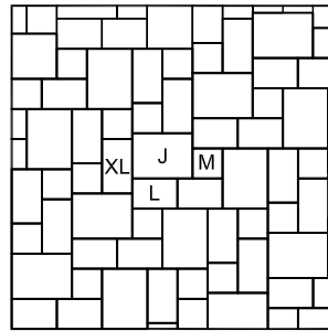
Pattern BE.23 - Medium 140x140mm - 10 Large 210x140mm - 6 XLarge 252x140mm - 6 Jumper 280x210mm - 6
