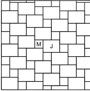
Pattern BE.17 - Medium 140x140mm - 13 Jumper 280x210mm - 13
