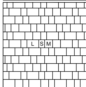
Pattern BE.27 - Small 105x140mm - 16 Medium 140x140mm - 16 Large 210x140mm - 16
